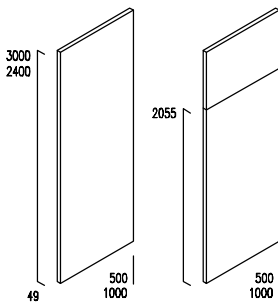
Forrado técnico vertical ciego Vertical technical solid cladding Doublage technique vertical plein
