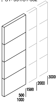
Forrado técnico horizontal ciego Horizontal technical solid cladding Doublage technique horizontal plein
