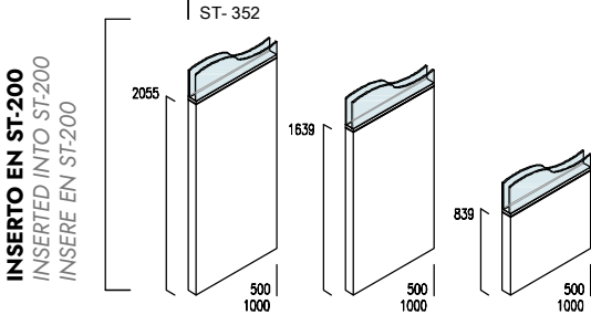
Tabique vertical ciego Vertical solid wall Cloison verticale pleine
