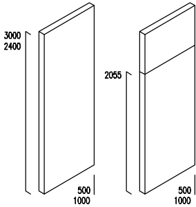
Forrado técnico vertical ciego Vertical technical solid cladding Doublage technique vertical plein
