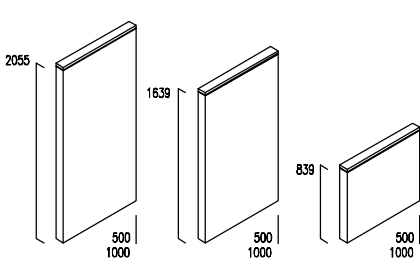
Tabique vertical ciego Vertical solid wall Cloison vertical pleine
